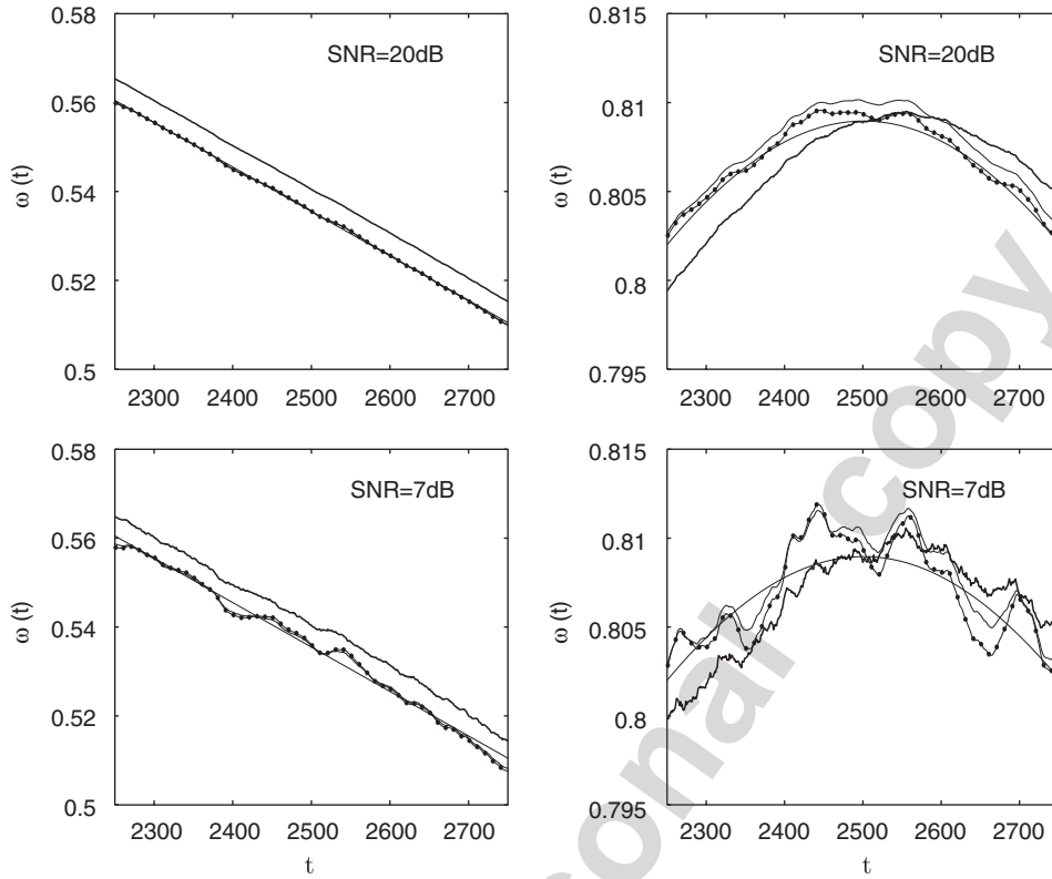
Fig. 1. True signal frequency changes (thin lines) and typical trajectories of frequency estimates yielded by the GANF algorithm (thick lines), and by its frequency-debiased versions based on the first-order (medium-thick lines) and second-order (lines with dots) polynomial approximations.
