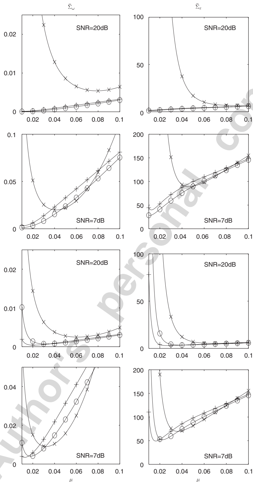
Fig. 2. Dependence of the averaged sums of the squared frequency estimation errors \bar{\Sigma}_\omega and excess prediction errors \bar{\Sigma}_\epsilon on the adaptation gain \mu . Comparison involves the estimates yielded by the original GANF algorithm ( \times ) and by its frequency-debiased versions proposed in the paper, based on the first-order ( \circ ) and second-order ( + ) polynomial approximation. The top four plots corresponds to linear frequency changes and the bottom four plots—to sinusoidal changes. All plots were evaluated on a grid of 90 equidistant values of \mu .
