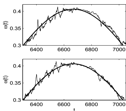
Fig. 2. True frequency changes (thick lines) and their estimates (thin lines) obtained using the pilot ANF filter ( \hat{\omega}(t) , upper plot) and its debiased version ( \tilde{\omega}(t) , lower plot).
