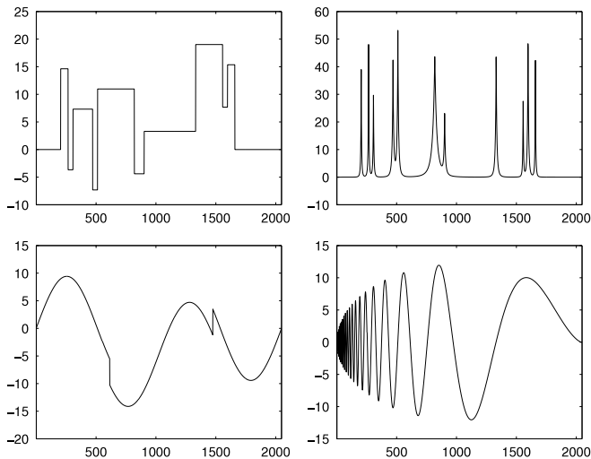
Fig. 1. Test signals: Blocks (top left), Bumps (top right), HeaviSine (bottom left), and Doppler (bottom right).
