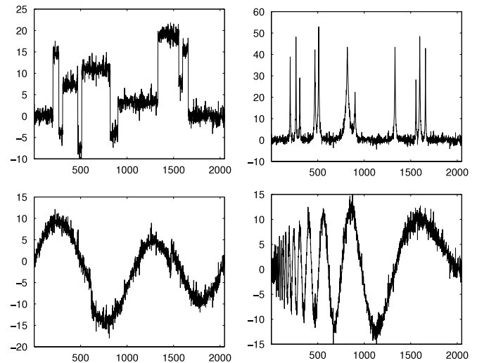
Fig. 4. Test signals with white Laplacian noise, \sigma_v^2 = 1 , SNR = 16.9 dB (SD(s)/ \sigma_v = 7 ).
