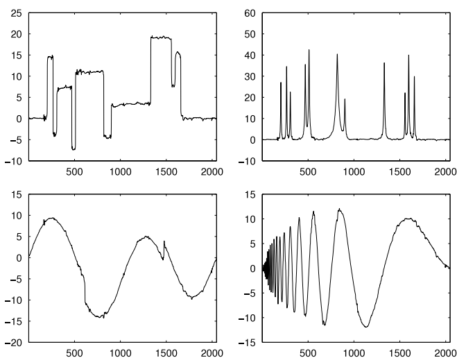
Fig. 3. Denoised test signals (Gaussian noise, C_3 ).
