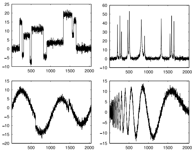
Fig. 2. Test signals with white Gaussian noise, \sigma_v^2 = 1 , SNR = 16.9 dB (SD(s)/ \sigma_v = 7 ).
